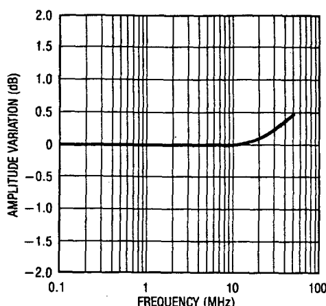
Figure 4's Response vs Frequency—250 Input
