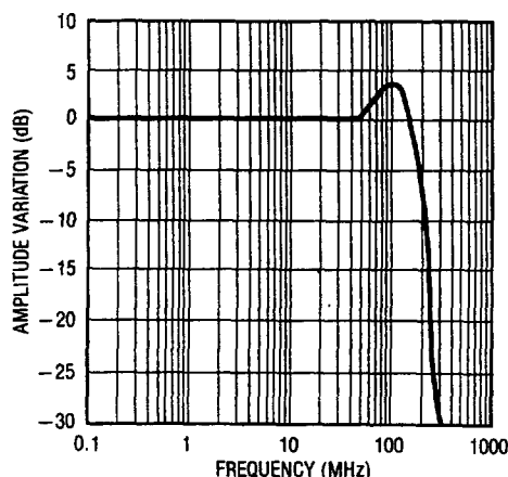
Figure 4's Response vs Frequency—500 Input
