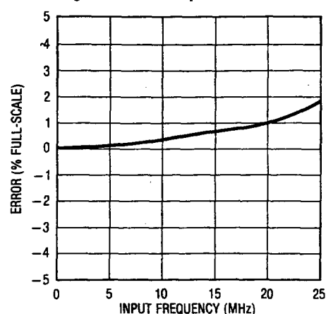
Accuracy vs Frequency for Figure 4—250 Input
