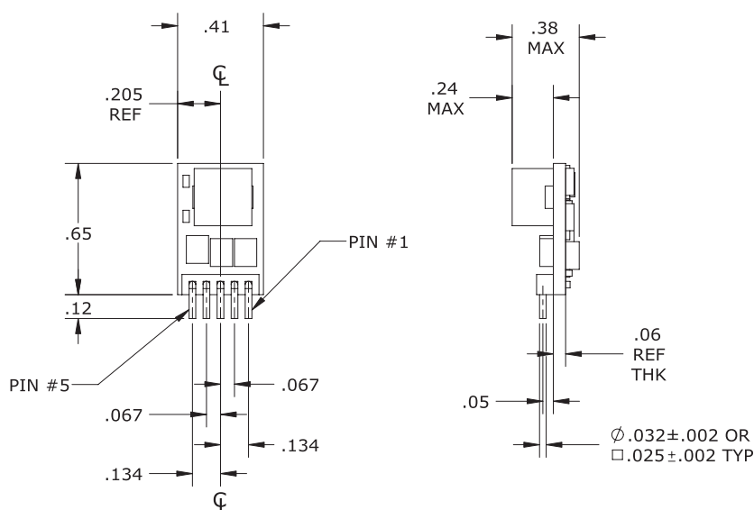
Figure 2 . LSS-T/10-W12 Series Component locations are typical.
