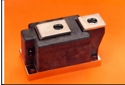
LS43__50 Single SCR POW-R-BLOK™ Module 500 Amperes / Up to 1600 Volts
