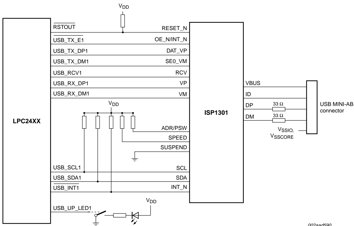
Fig 16. LPC2470 USB OTG port configuration: VP_VM mode
