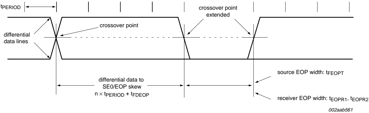
Fig 10. Differential data-to-EOP transition skew and EOP width
