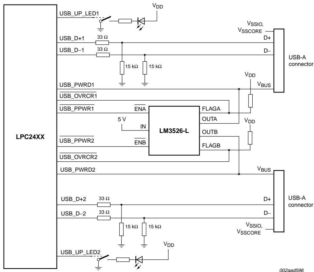
Fig 18. LPC2470 USB OTG port configuration: USB port 1 host, USB port 2 host
