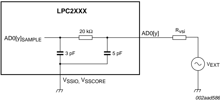
Fig 6. Suggested ADC interface - LPC2470 AD0[y] pin
