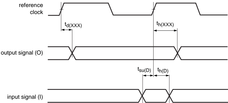
Fig 12. Signal timing
