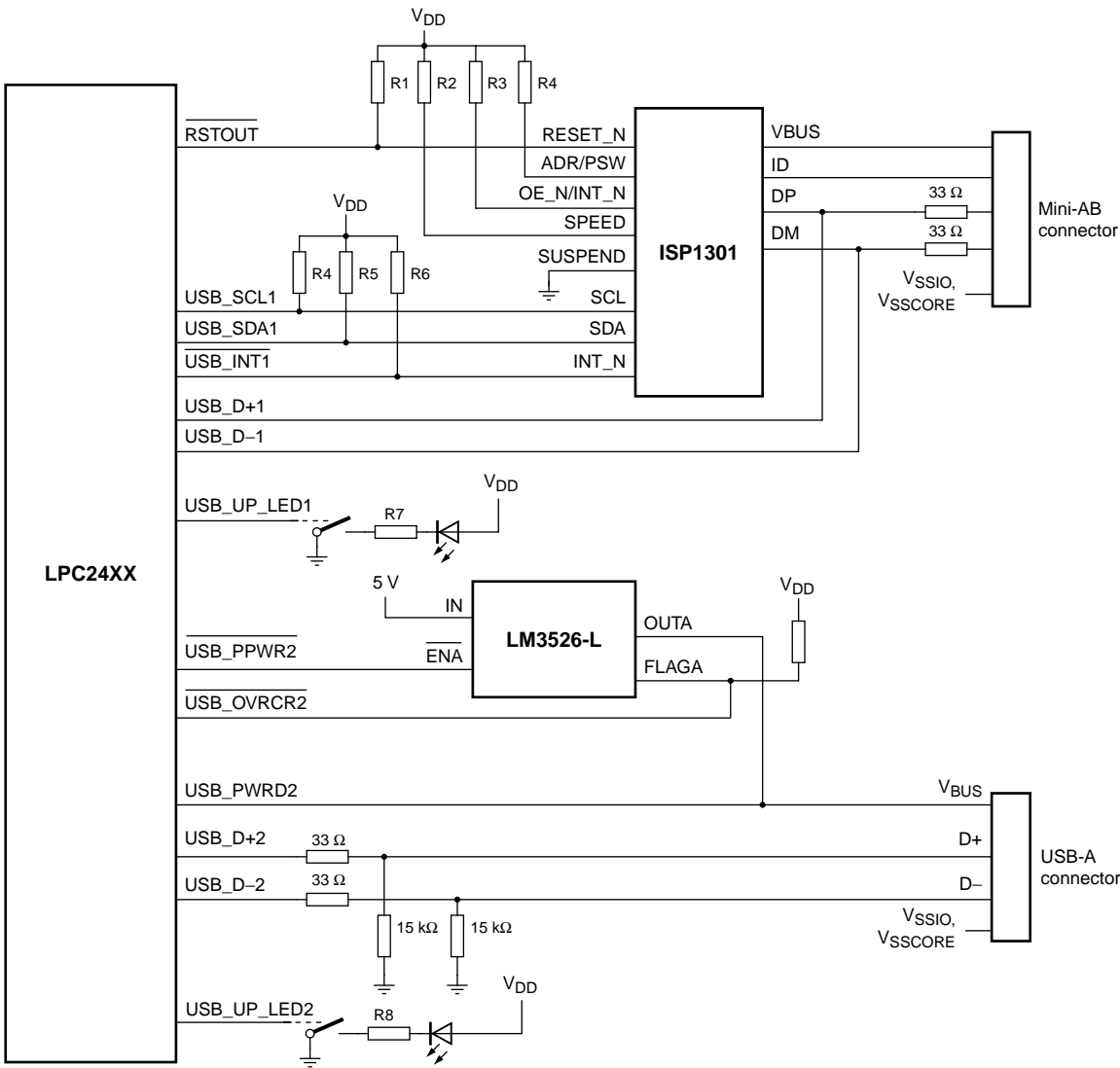
Fig 15. LPC2470 USB OTG port configuration: USB port 1 OTG dual-role device, USB port 2 host
