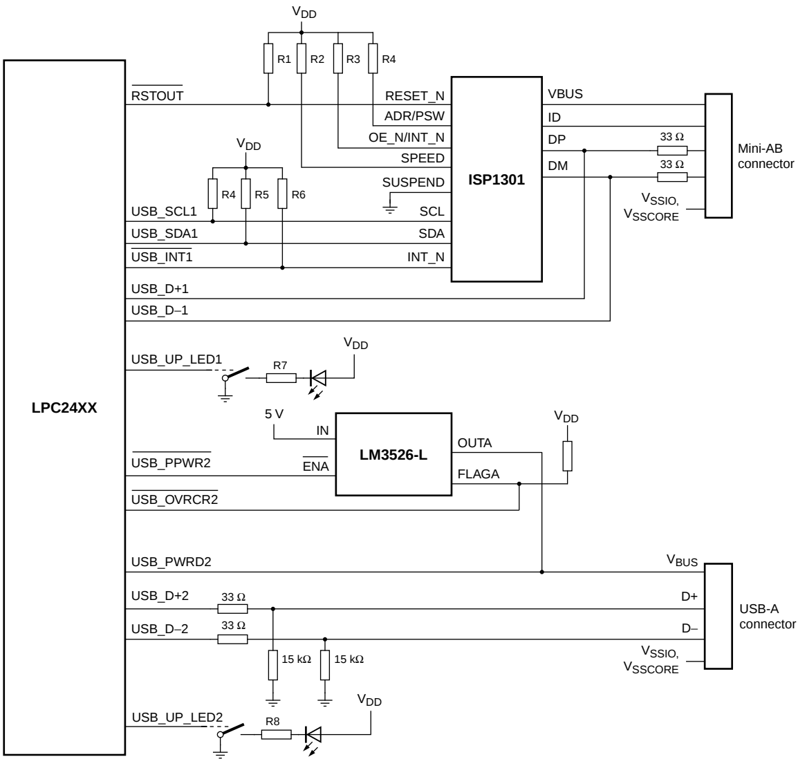
Fig 15. LPC2468 USB OTG port configuration: USB port 1 OTG dual-role device, USB port 2 host
