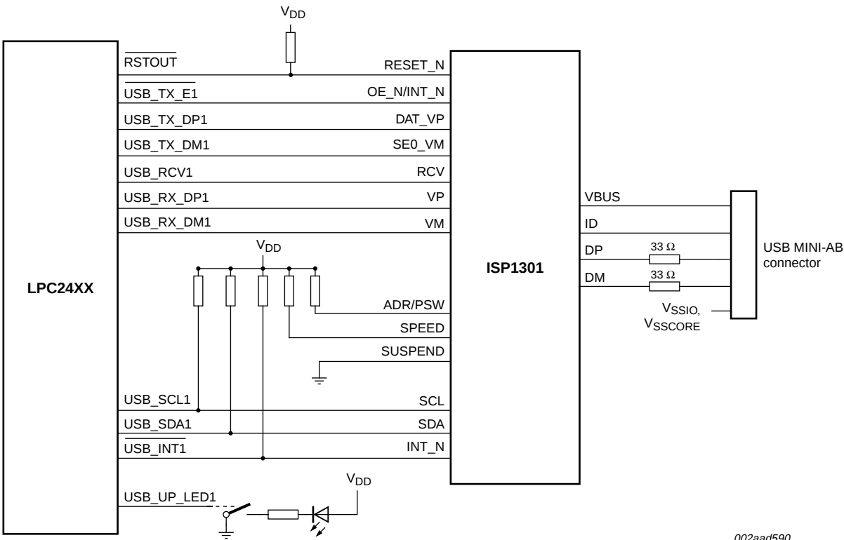
Fig 16. LPC2468 USB OTG port configuration: VP_VM mode
