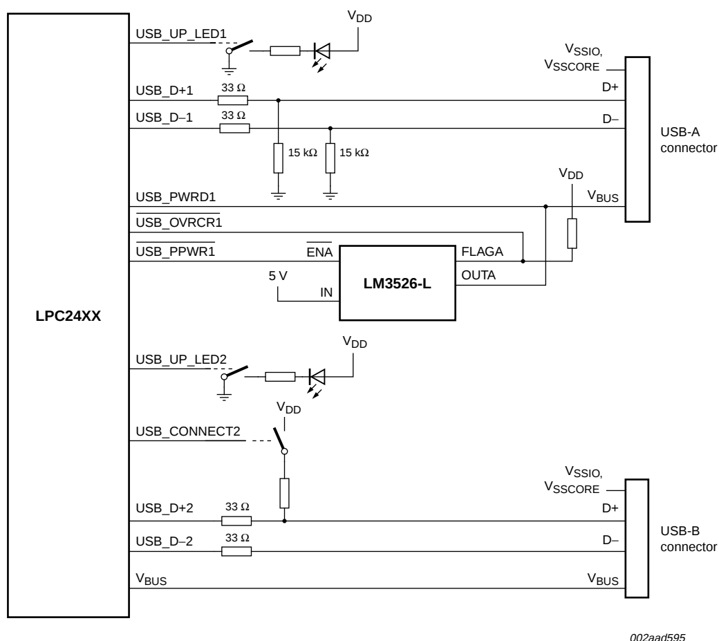
Fig 17. LPC2468 USB OTG port configuration: USB port 2 device, USB port 1 host
