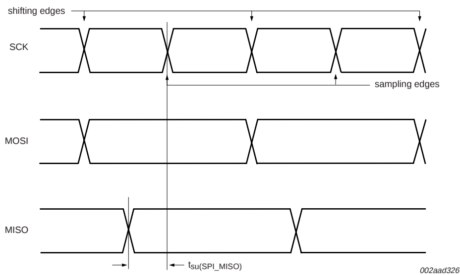
Fig 11. MISO line set-up time in SSP Master mode
