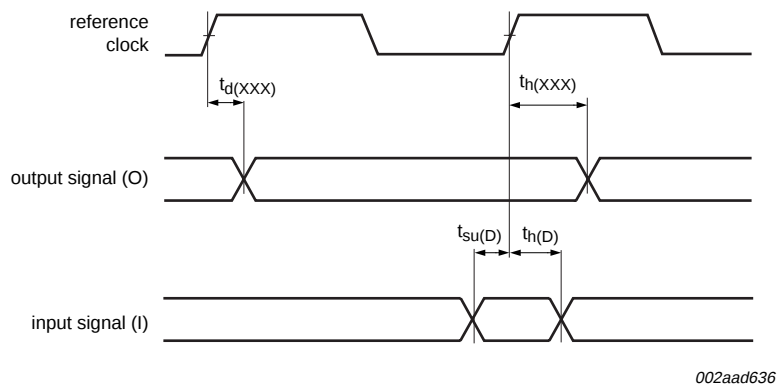
Fig 12. Signal timing
