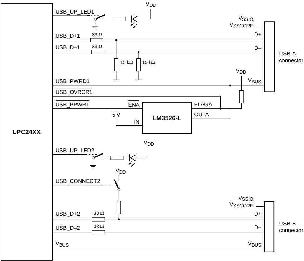
Fig 17. LPC2420/2460 USB OTG port configuration: USB port 2 device, USB port 1 host
