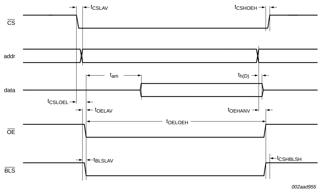
Fig 10. External memory read access
