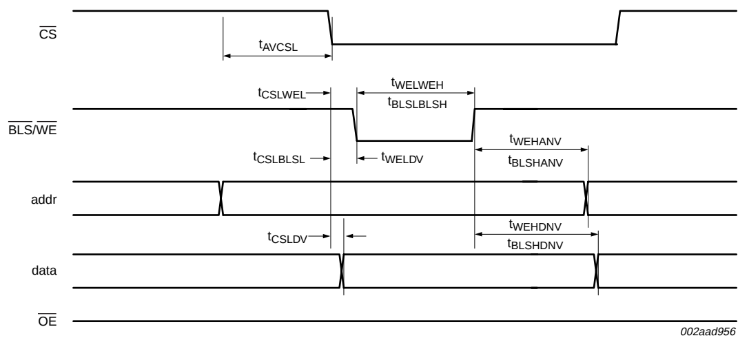
Fig 11. External memory write access
