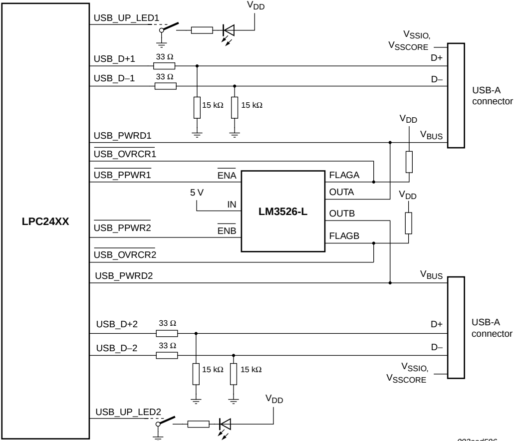
Fig 18. LPC2420/2460 USB OTG port configuration: USB port 1 host, USB port 2 host
