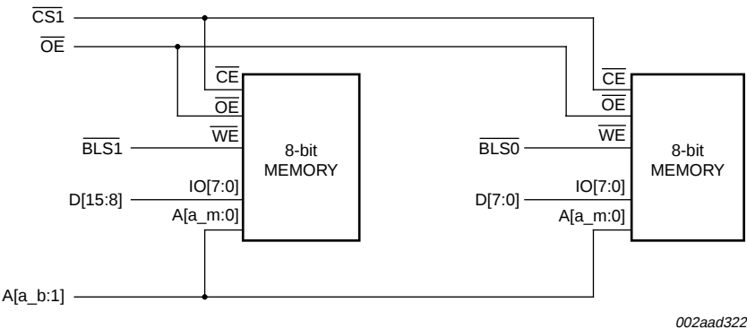
Fig 19. Booting from two 8-bit memory chips
