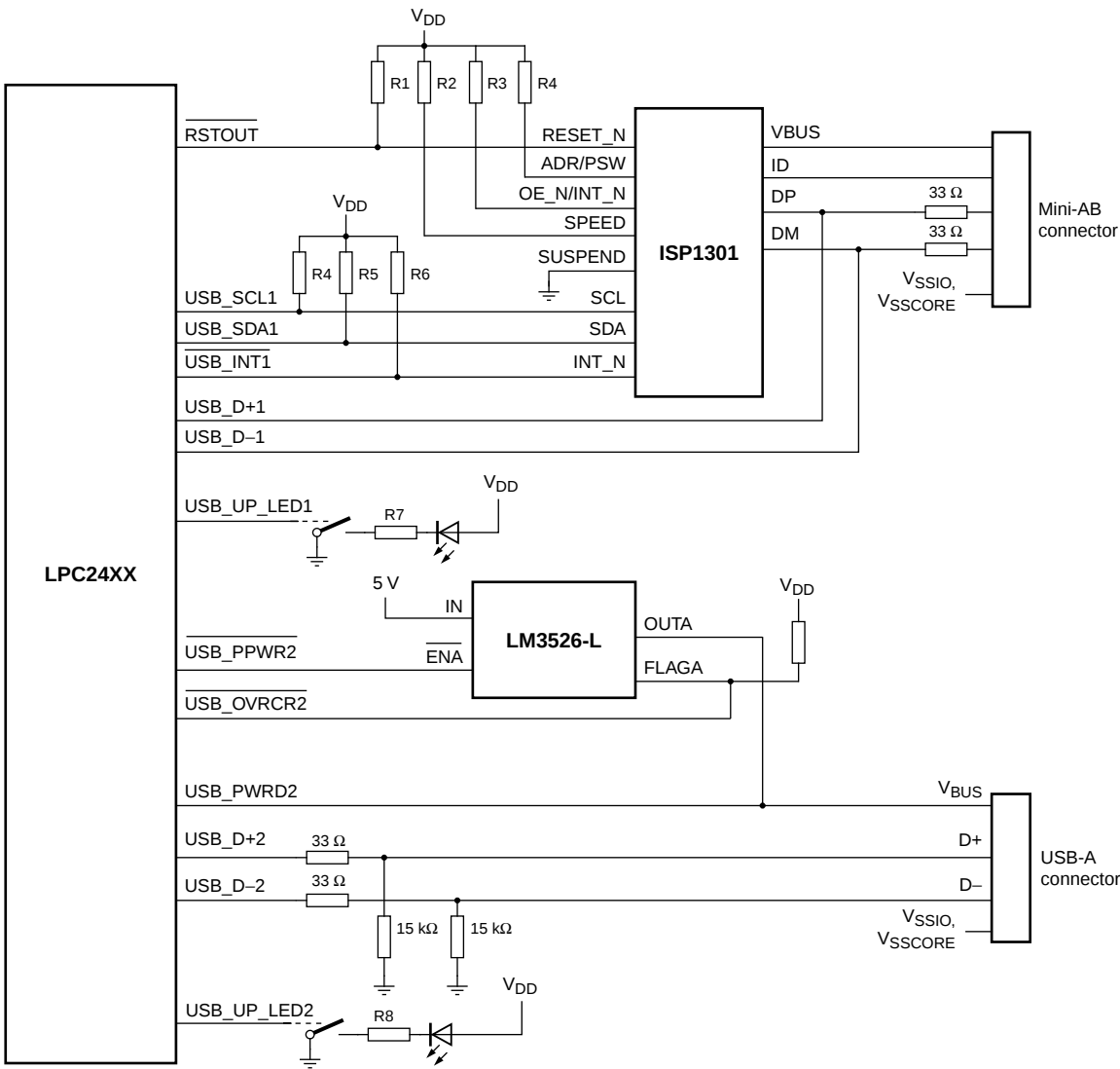
Fig 15. LPC2420/2460 USB OTG port configuration: USB port 1 OTG dual-role device, USB port 2 host
