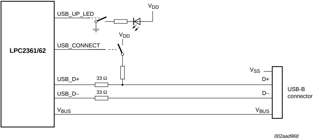
Fig 13. LPC2361/62 USB device port configuration
