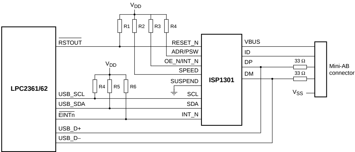
Fig 11. LPC2361/62 USB OTG port configuration
