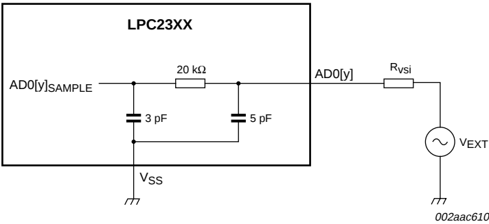
Fig 5. Suggested ADC interface - LPC2361/62 AD0[y] pin
