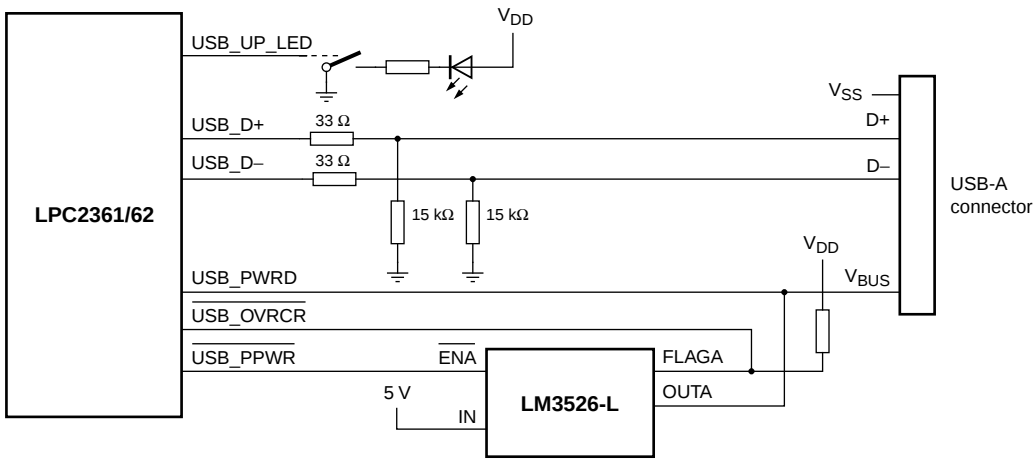
Fig 12. LPC2361/62 USB host port configuration
