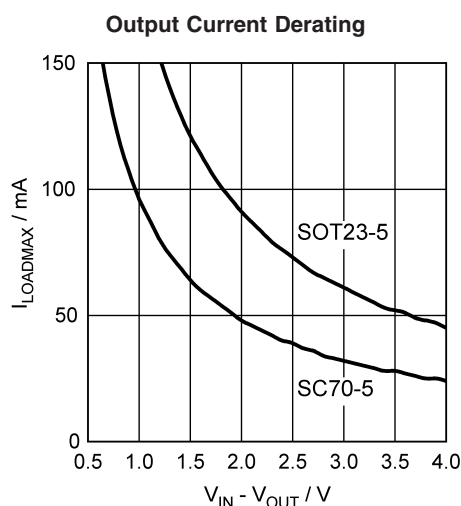
FIGURE 6: Maximum Load Current vs ( V_{IN} - V_{OUT} ), T_A = 85^\circ\text{C} , V_{OUT} = 1.5\text{V}
