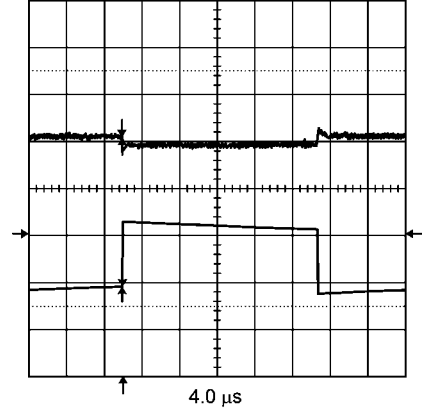
LDO1 Load Transient V_{IN} = 4.1 volts V_{OUT} = 1.8 volts no-load-100 mA
