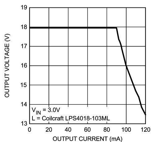
Boost Output Voltage vs. Current
