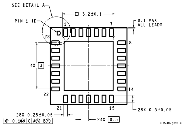
28 Lead LLP Package NS Package Number lqa28A
