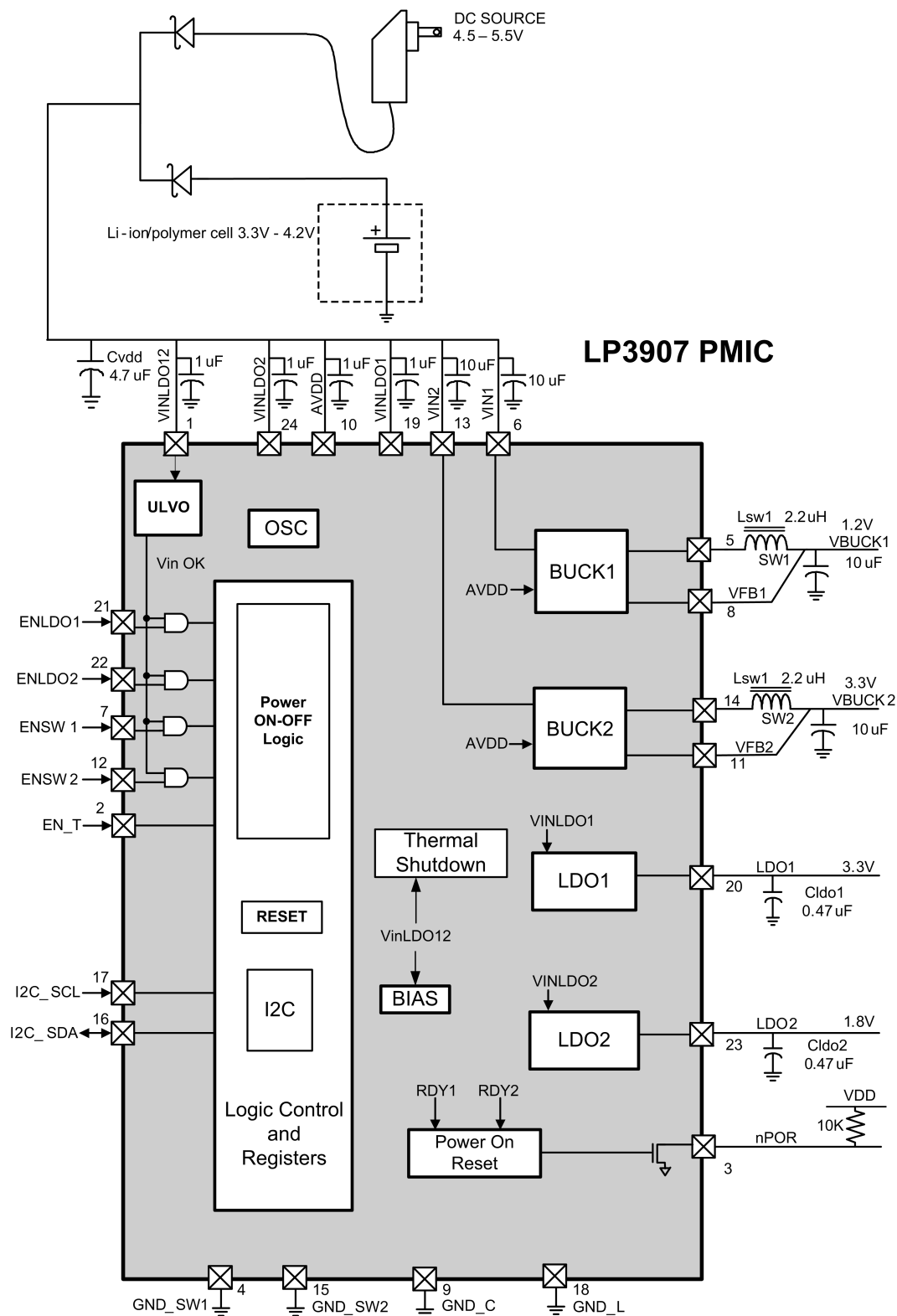
FIGURE 2. Application Circuit
