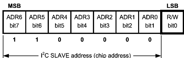
I 2 C Chip Address (see note above)
