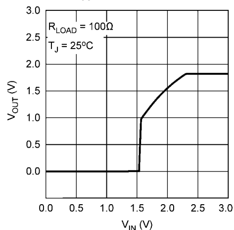
V OUT vs V IN (1.8V)
