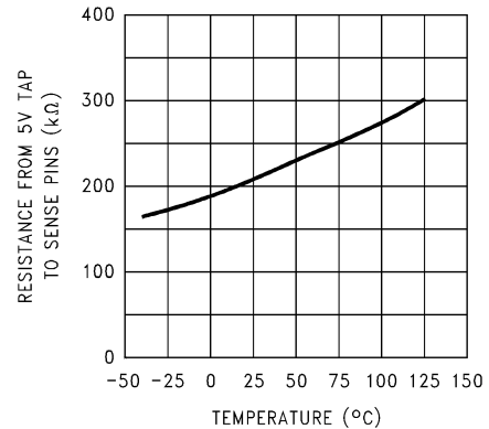
Divider Resistance
