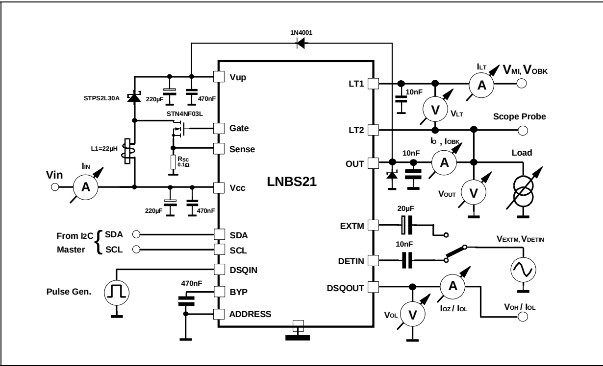
Figure 7: Test Circuit
