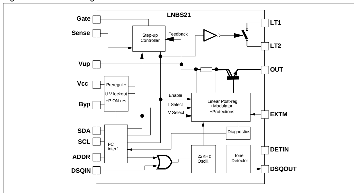
Figure 1: Schematic Diagram
