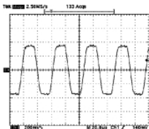
Figure 34: 22kHz Tone
