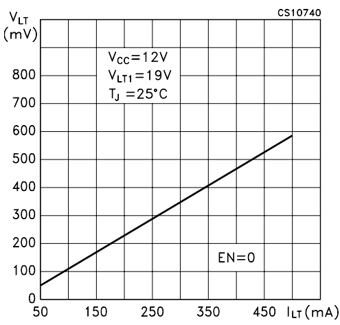
Figure 28: Loophthrough Switch Drop Voltage vs Loophthrough Current
