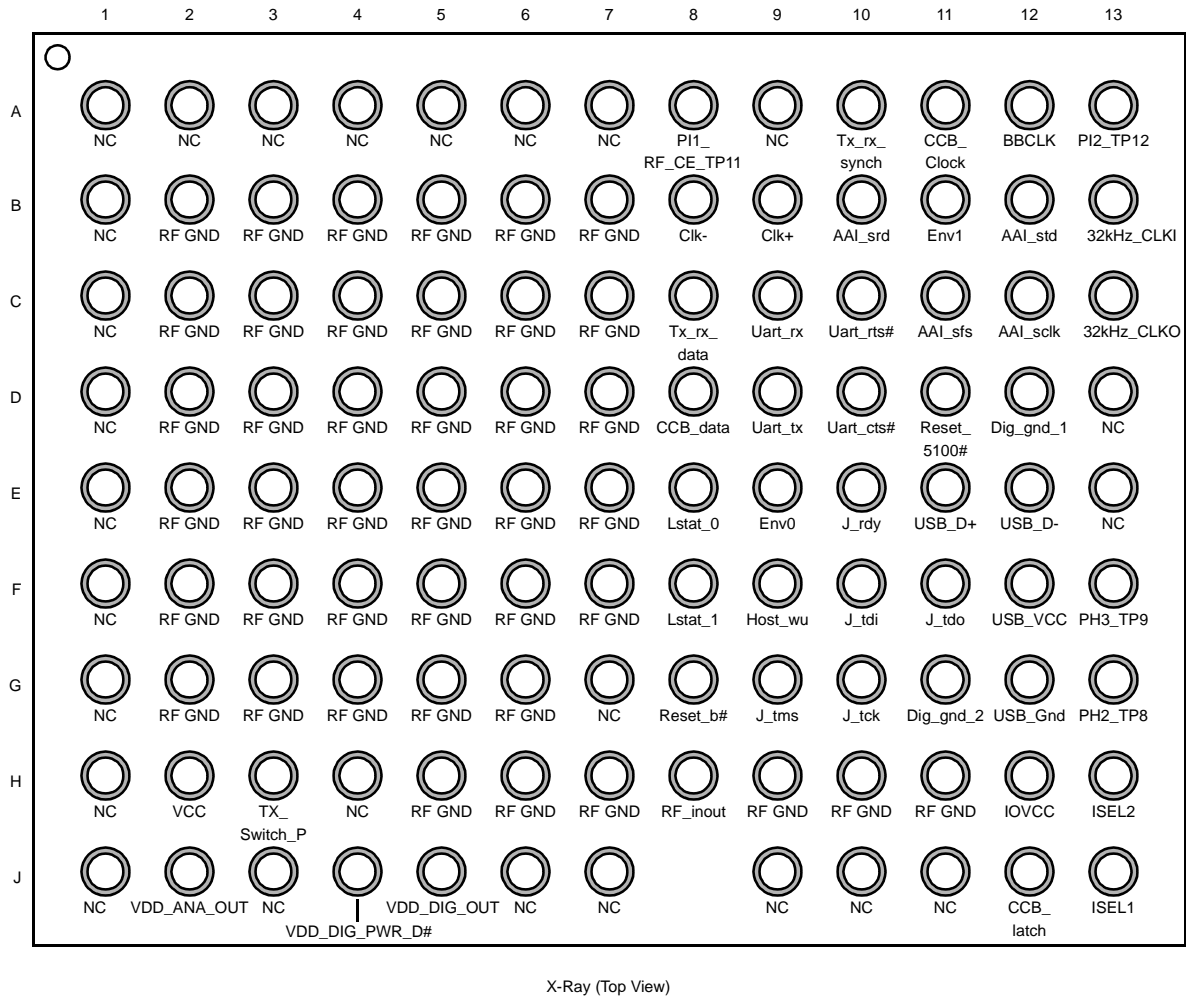
Figure 1. Connection Diagram
