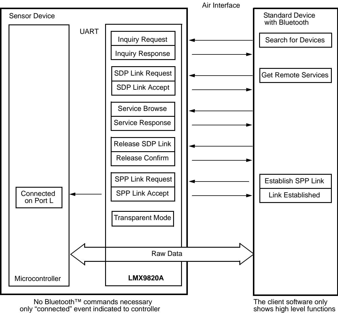
Figure 21. Point-to-Point Connection
