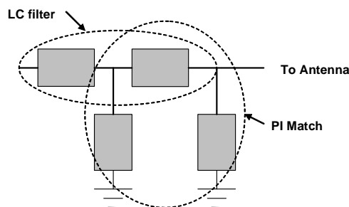
Figure 15. Front End Layout
