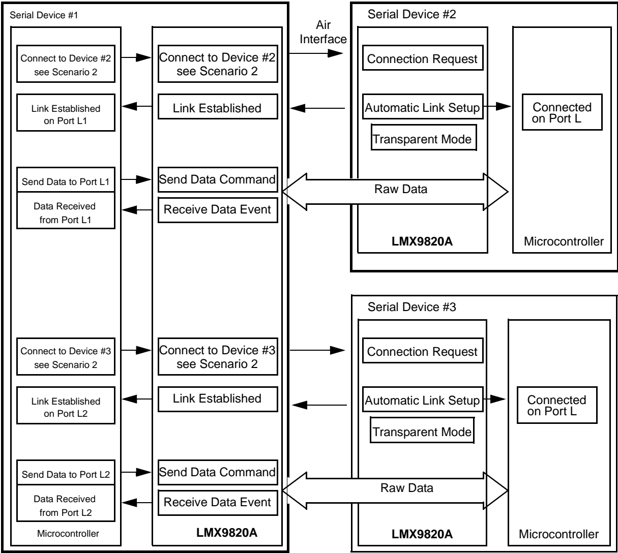
Figure 23. Point-to-Multipoint Connection
