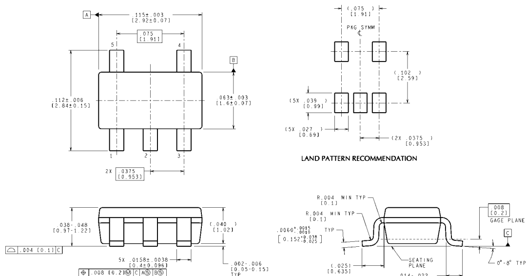
5-Pin SOT-23 NS Package Number MF05A
