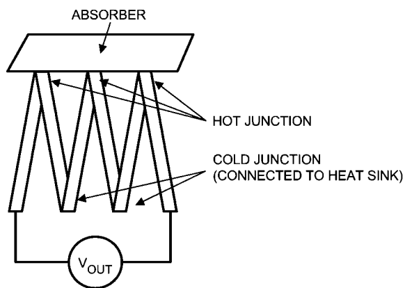
FIGURE 7. Thermopile
