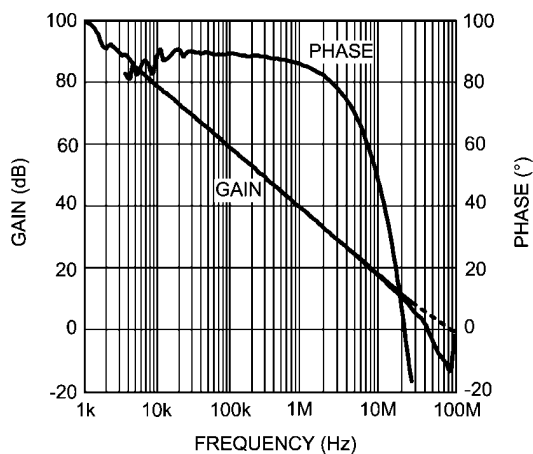
FIGURE 1. LMP7717 A_{VOL} vs. Frequency
