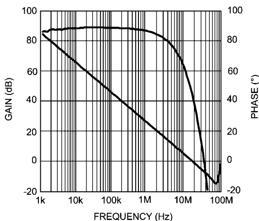
FIGURE 2. LMP7715 A_{VOL} vs. Frequency
