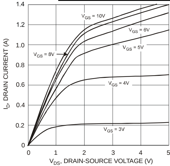
Fig. 10 Output Characteristics
