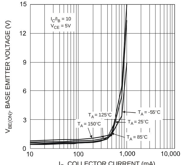
Fig. 8 V_{BE(ON)} vs. I_C @ V_{CE} = 5V
