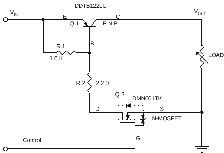
Fig. 20 Circuit Diagram
