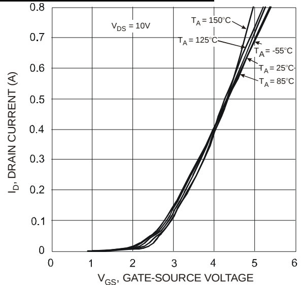
Fig. 11 Transfer Characteristics
