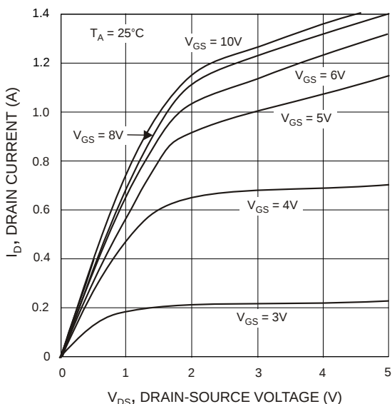
Fig. 10 Output Characteristics
