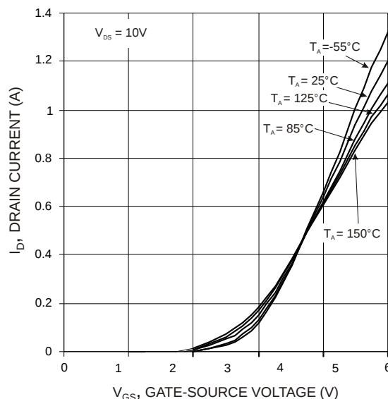
Fig. 11 Transfer Characteristics
