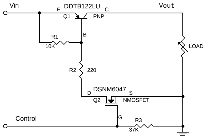
Fig 20 : Circuit Diagram
