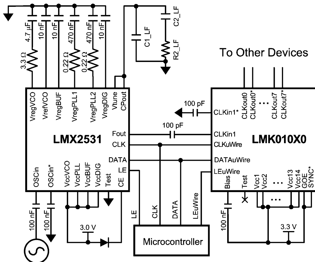
FIGURE 1. Typical Application
