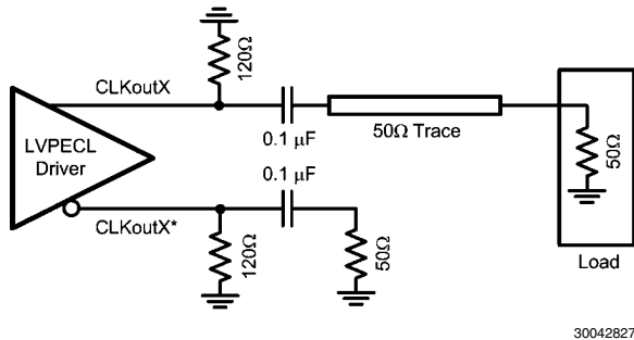
FIGURE 10. Single-Ended LVPECL Operation, AC Coupling
