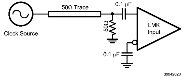
FIGURE 11. Single-Ended Sine Wave Input
