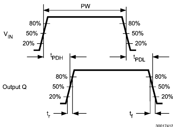
FIGURE 9. Propagation Delay
