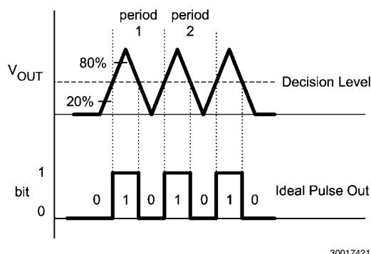
FIGURE 18. Bit Rates
