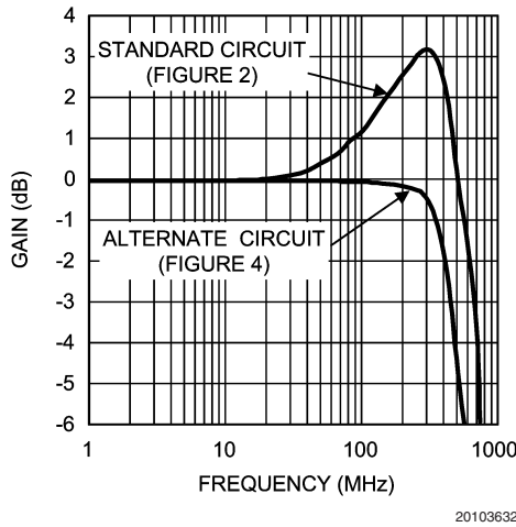
FIGURE 5. Unity Gain Frequency Response
