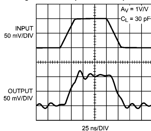
Medium Signal Pulse Response with Capacitive Load
