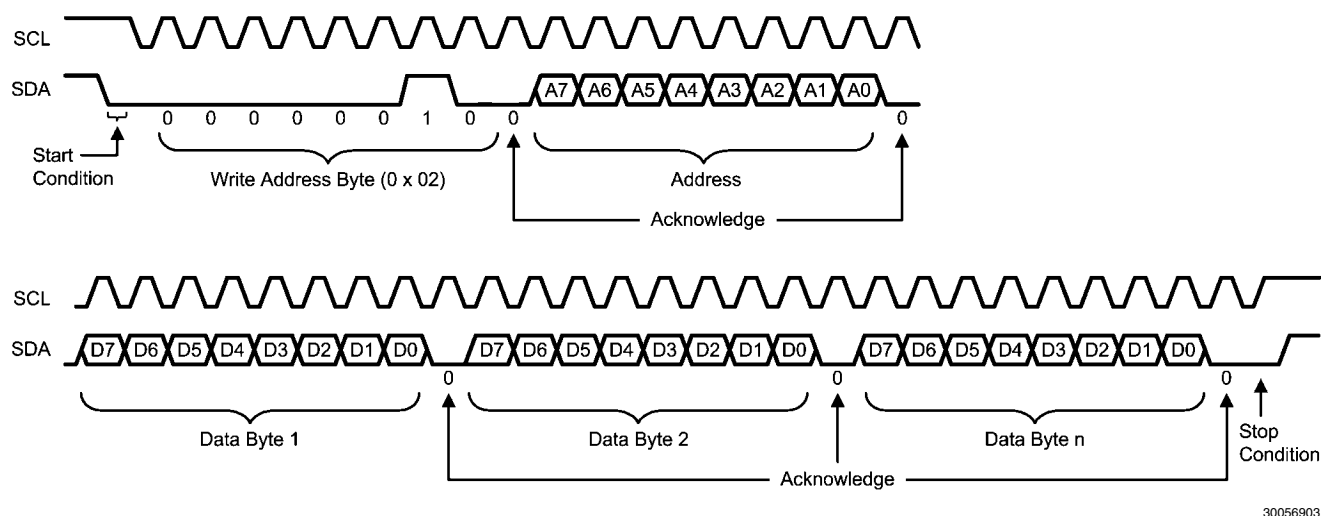
FIGURE 7. LMH6586 Write Sequence
