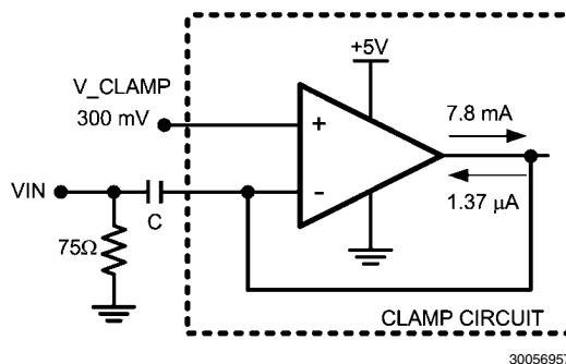
FIGURE 5. Clamp Circuit
