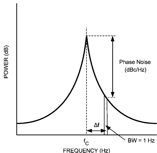
FIGURE 4. Phase Noise
