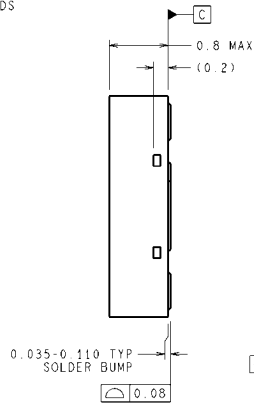
8-Pin LLP NS Package Number YDA08A
