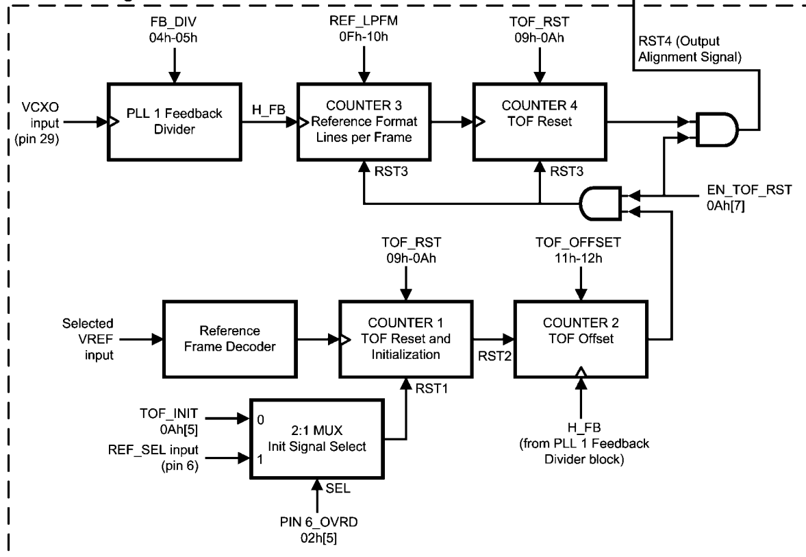
FIGURE 3. Functional Block Diagram – TOF Generation and Output Initialization Circuitry
