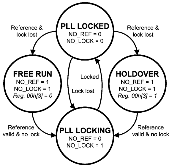
FIGURE 1. Genlock Mode State Diagram
