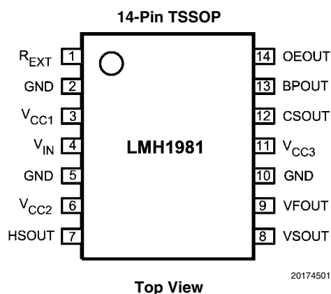
FIGURE 1. Pinout
