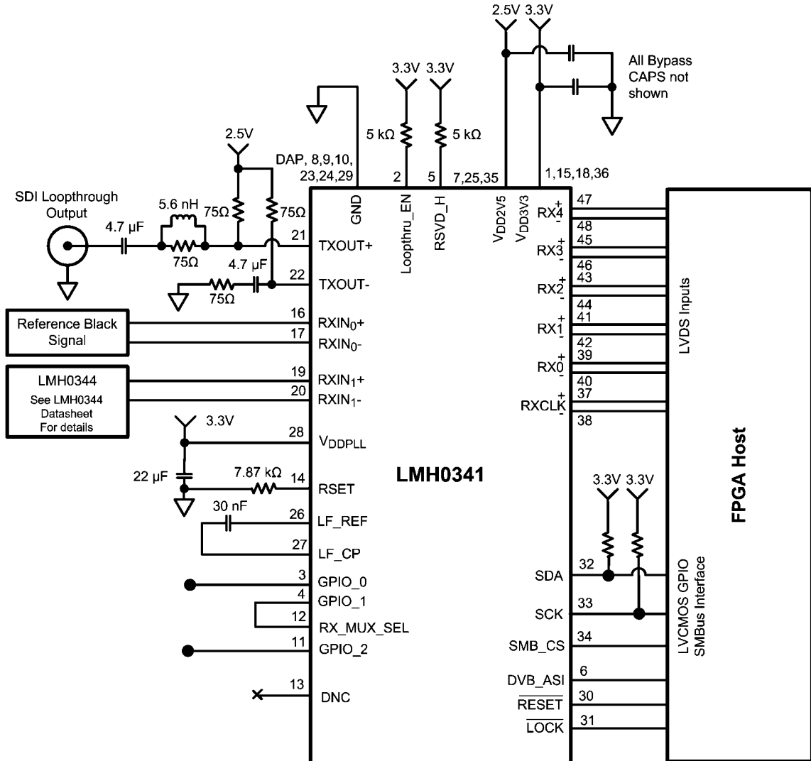
FIGURE 15. Typical SMPTE Application Circuit
