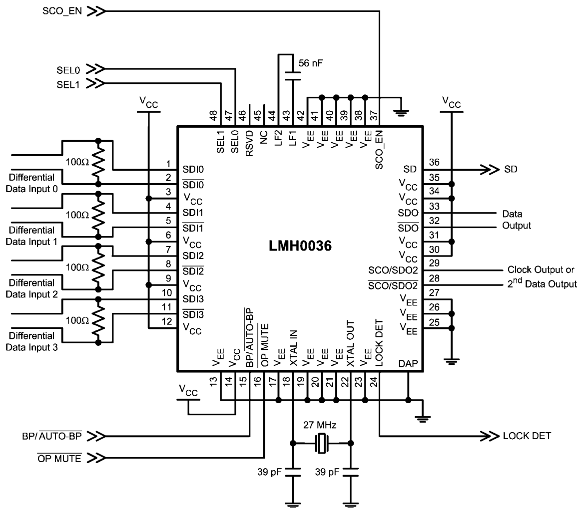
FIGURE 4. Application Circuit
