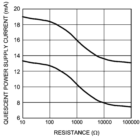
Quiescent Current vs Bandwidth Control Resistance V_S = \pm 15V (Bottom) & V_S = \pm 22V (Top)
