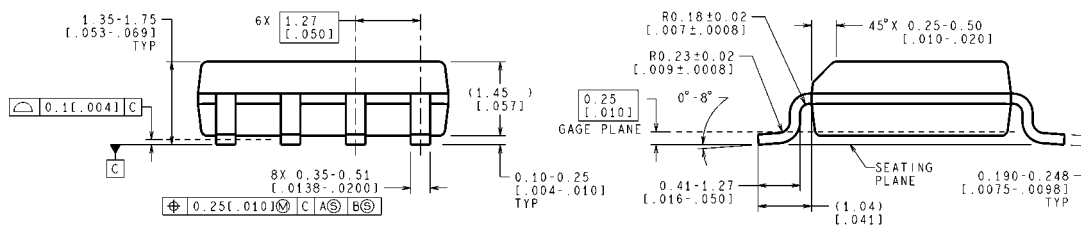
8-Pin SOIC NS Package Number M08A
