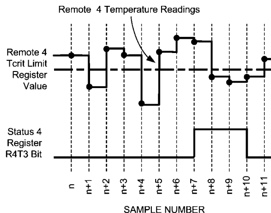
FIGURE 4. Fault Queue Response Diagram (with 0°C hysteresis)
