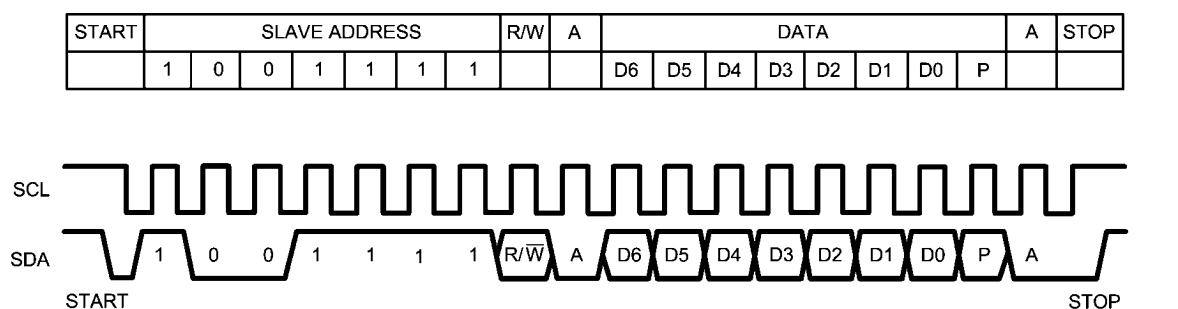
FIGURE 6. Timing Diagram
