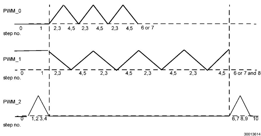
FIGURE 14. PWM Outputs
