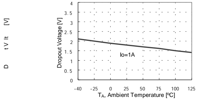
Figure 4. Dropout Voltage
