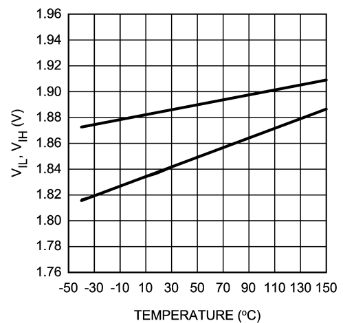
Input Threshold vs Temperature
