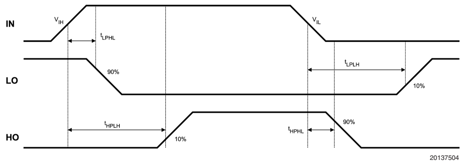
FIGURE 3. LM5105 Switching Time Definitions: t_{LPLH} , t_{LPHL} , t_{HPLH} , t_{HPHL}
