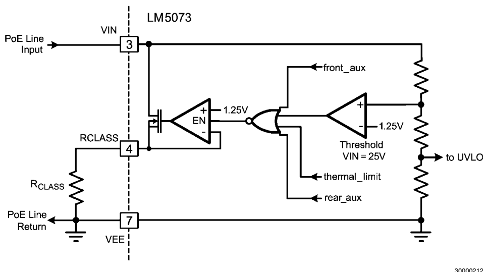
FIGURE 4. PD Classification – Fulfilled With a Single External Resistor
