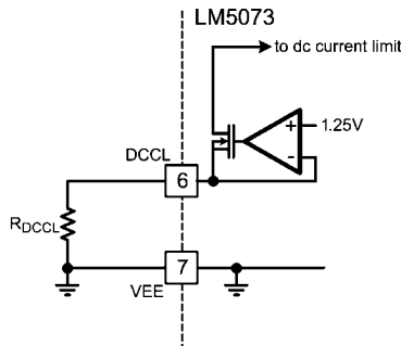
FIGURE 6. Input DC Current Limit Programming via R_{DCCCL}
