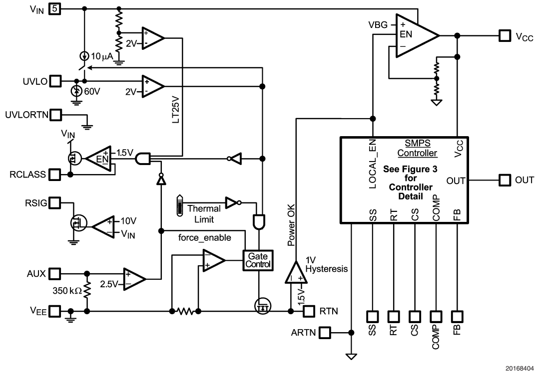
FIGURE 2. Top Level Block Diagram
