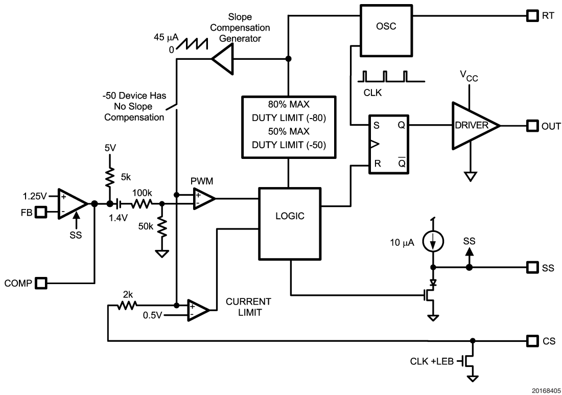
FIGURE 3. PWM Controller Block Diagram
