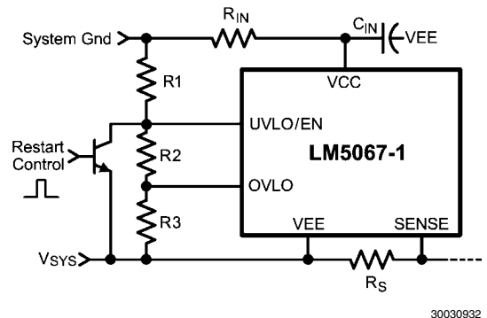
FIGURE 5. Latched Fault Restart Control
