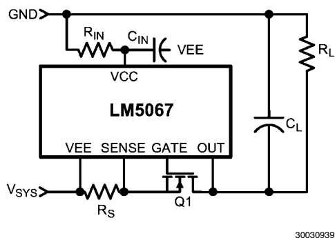
FIGURE 9. Load Draws Current During Turn-On
