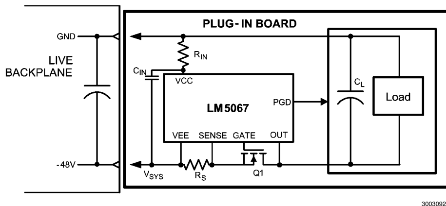
FIGURE 2. LM5067 Application
