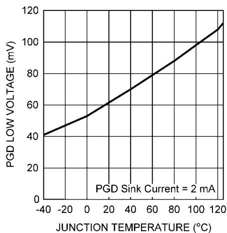
PGD Pin Low Voltage vs. Temperature
