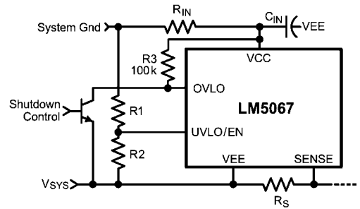
b) Shutdown/Enable Using the OVLO Pin
