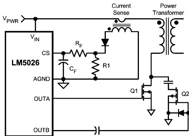
FIGURE 15. Current Sense Using a Current Sense Transformer
