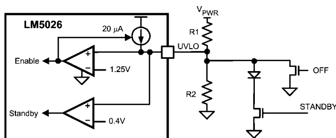
FIGURE 14. Remote Standby and Disable Control
