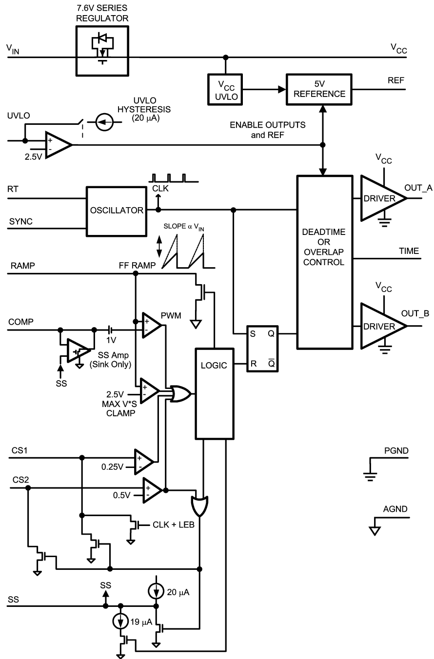
Simplified Block Diagram
