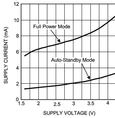
Supply Current vs Supply Voltage Z_L = 2\mu F + 30\Omega
