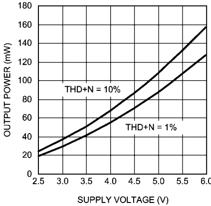
Output Power vs Supply Voltage R_L = 32\Omega , Mode 7, SE
