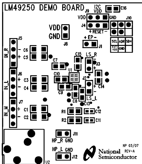
Top Silkscreen
