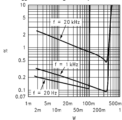
THD+N vs Output Power V_{DD} = 3V , BTL, R_L = 8\Omega , A_V = 8\text{ dB}
