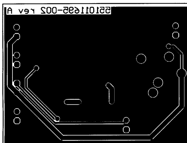
FIGURE 7. Bottom Layer
