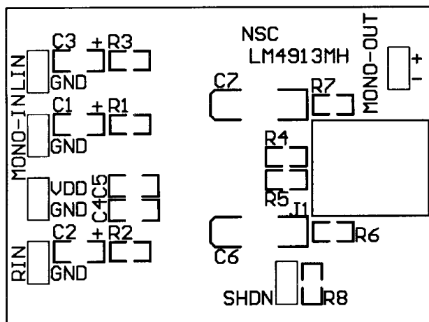
FIGURE 5. Top Overlay
