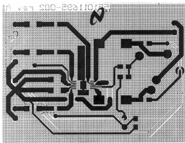
FIGURE 8. Composite Layer
