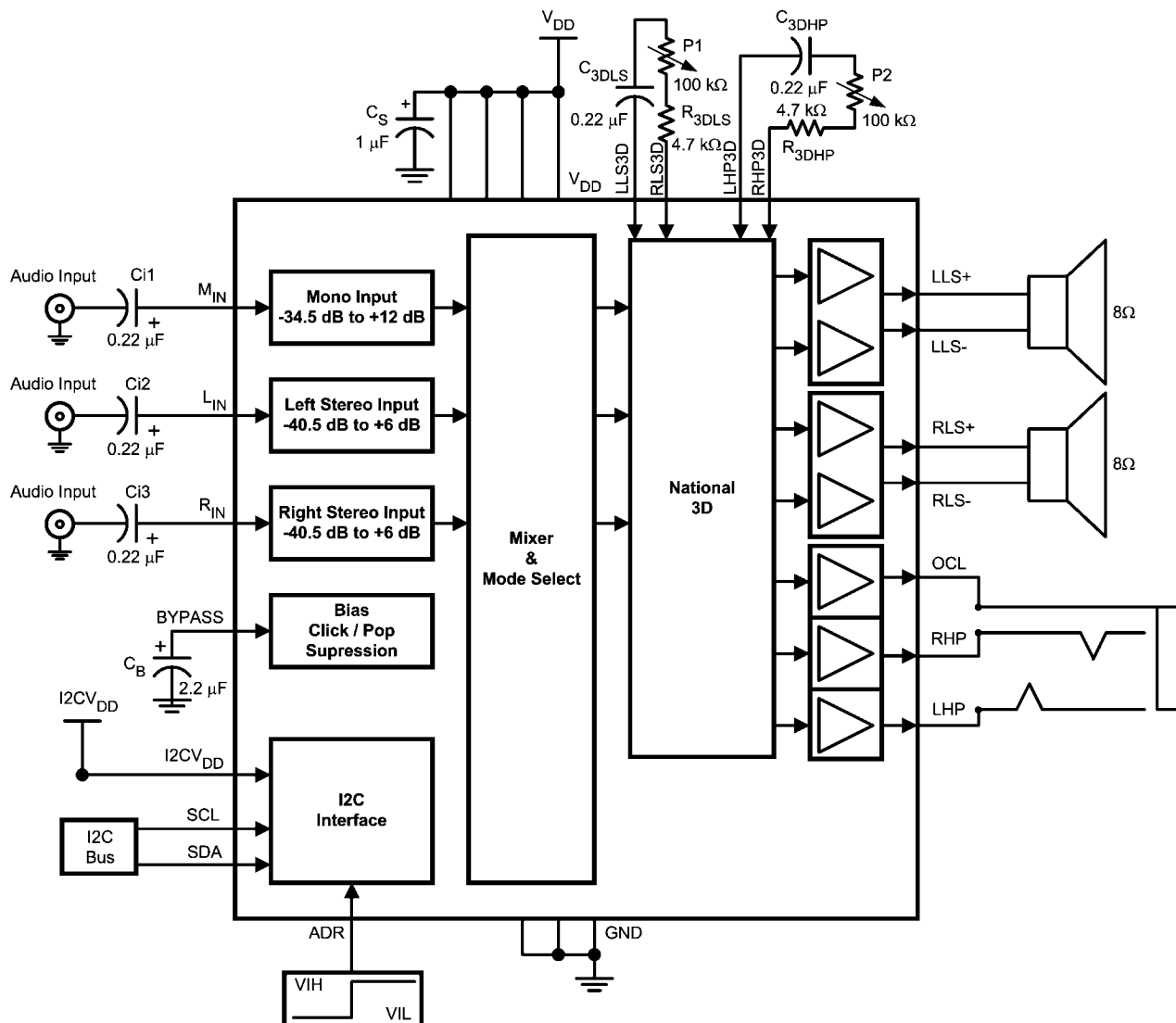
FIGURE 1. Audio Sub-System Block Diagram
