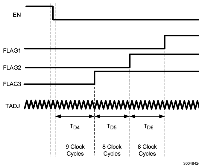
FIGURE 5. Power Down Sequence, INV High
