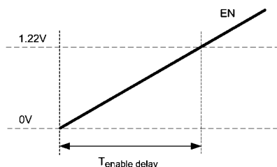
FIGURE 7. Enable Delay Timing
