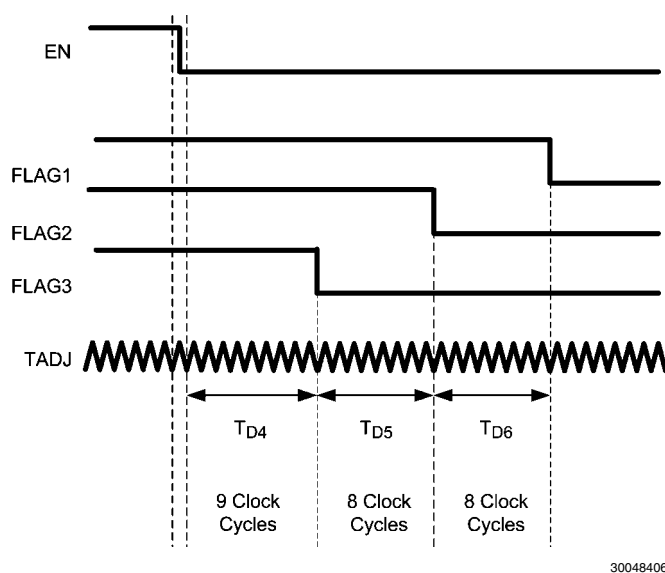
FIGURE 4. Power Down Sequence, INV Low
