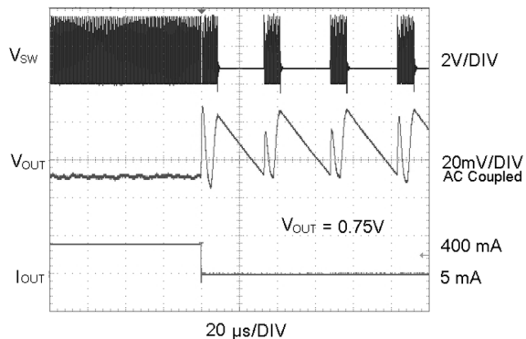
Load Transient Response ( V_{OUT} = 0.75V , PWM Mode to ECO Mode)
