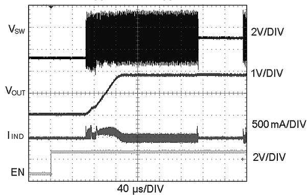
Start Up into ECO Mode ( V_{OUT} = 1.8V , R_{OUT} = 1.8\text{ k}\Omega )
