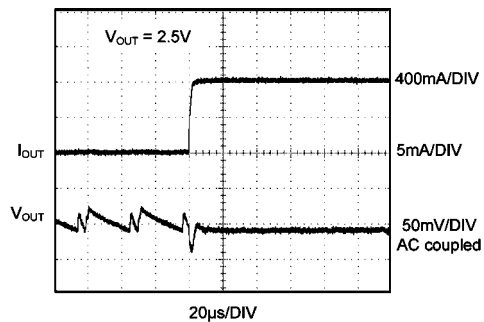
Load Transient Response ( V_{OUT} = 2.5V , ECO Mode to PWM Mode)
