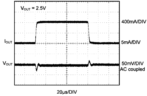
Load Transient Reponse ( V_{OUT} = 1.8V , FPWM Mode)
