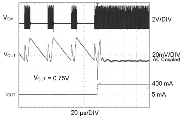
Load Transient Response ( V_{OUT} = 0.75V , ECO Mode to PWM Mode)
