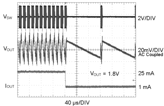
Load Transient Response ( V_{OUT} = 1.8V , ECO Mode 25 mA to 1mA)
