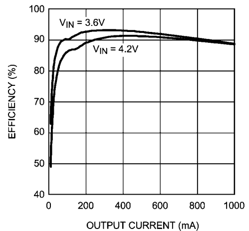
Efficiency vs. Output Current ( V_{OUT} = 2.5V , FPWM Mode)
