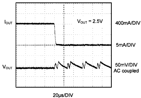
Load Transient Response ( V_{OUT} = 2.5V , ECO Mode to PWM Mode)
