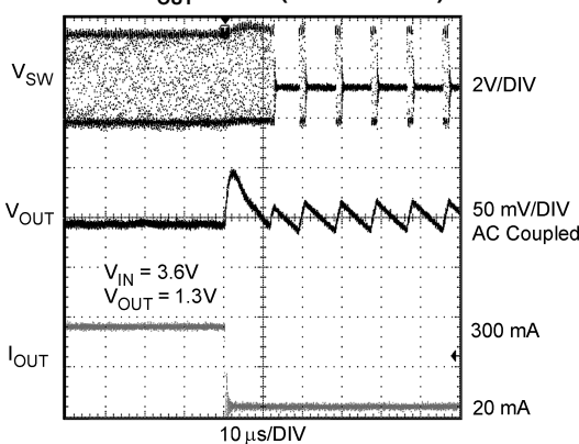
Mode Change by Load Transients V_{OUT} = 1.3V (PWM to PFM)
