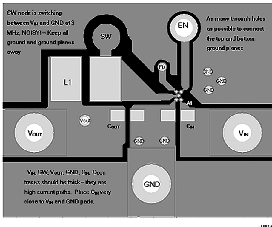
FIGURE 9. Board Layout Design Rules for the LM3677
