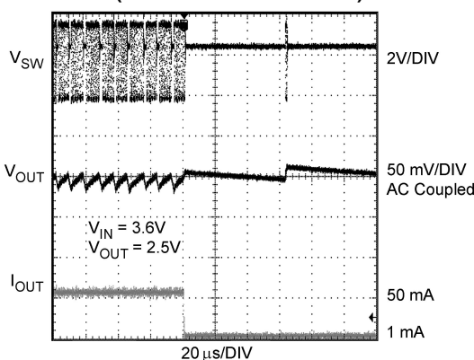
Load Transient Response ( V_{OUT} = 2.5V ) (PFM Mode 50mA to 1mA)
