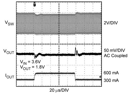
Load Transient Response V_{OUT} = 1.8V (PWM Mode)
