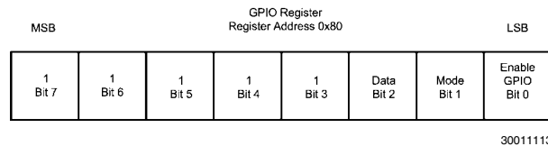
FIGURE 11. GPIO Register Description
