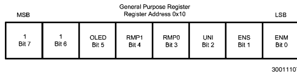
FIGURE 7. General Purpose Register Description
