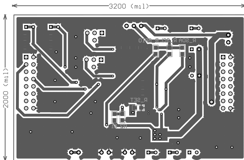
FIGURE 2. LM3509 Evaluation Board Layout (Top Side)
